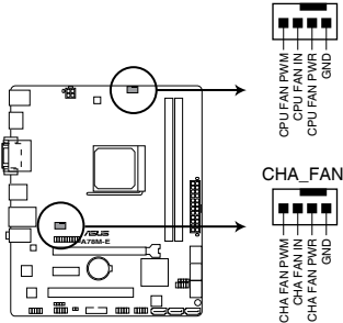
A78M-E Fan connectors
