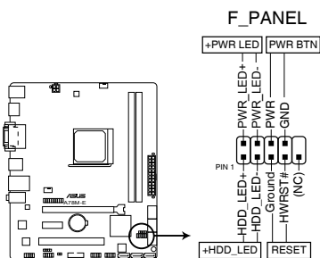
A78M-E System panel connector
