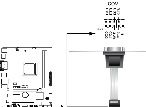
A78M-E Serial port connectors
