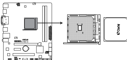
A78M-E CPU socket FM2+
