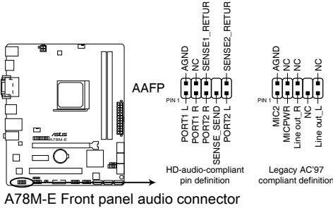
A78M-E Front panel audio connector
