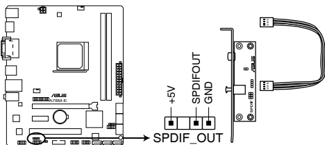
A78M-E Digital audio connector
