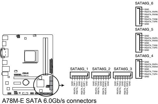
A78M-E SATA 6.0Gb/s connectors
