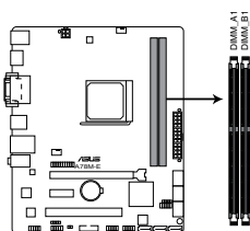
A78M-E 240-pin DDR3 DIMM sockets
